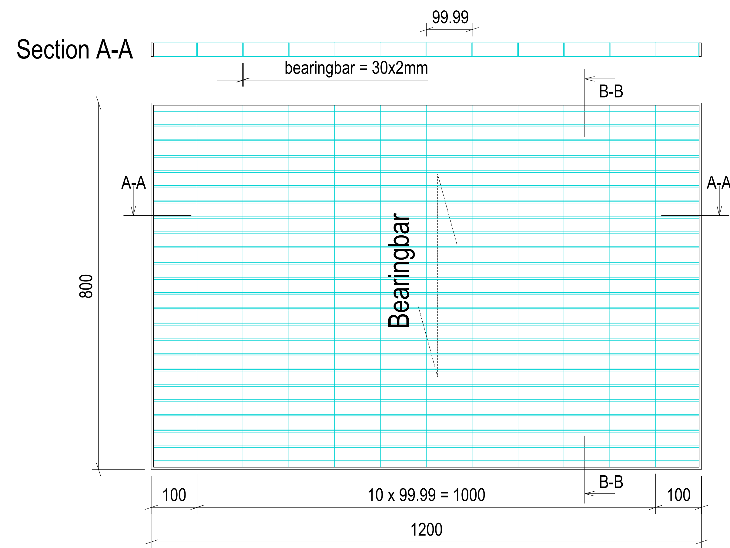
TYPE RL 30-2/ 99.99x33.33 Louvre 40-2/ 45°
