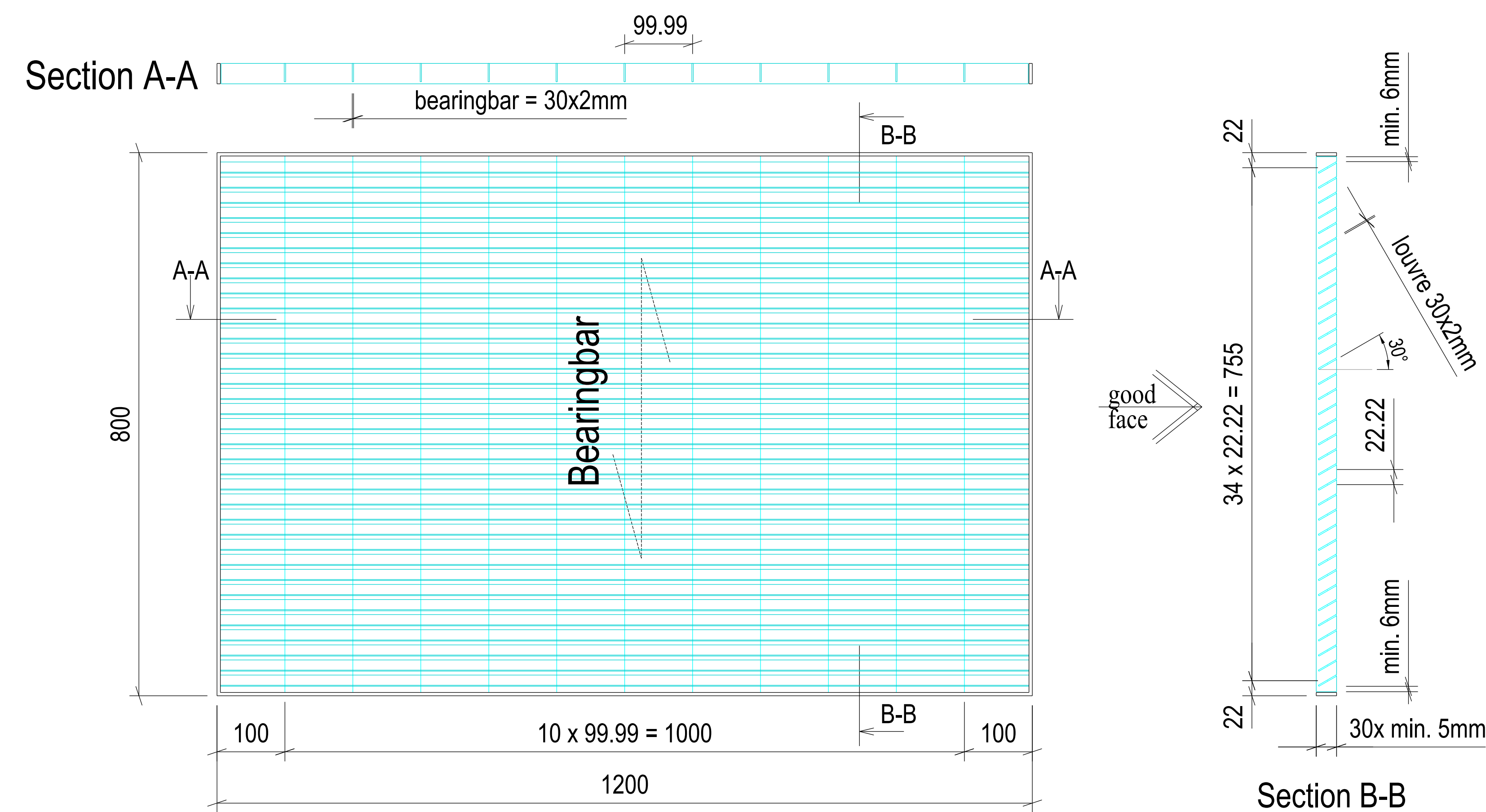
TYPE RL 30-2/ 99.99x22.22 Louvre 30-2/ 30°
