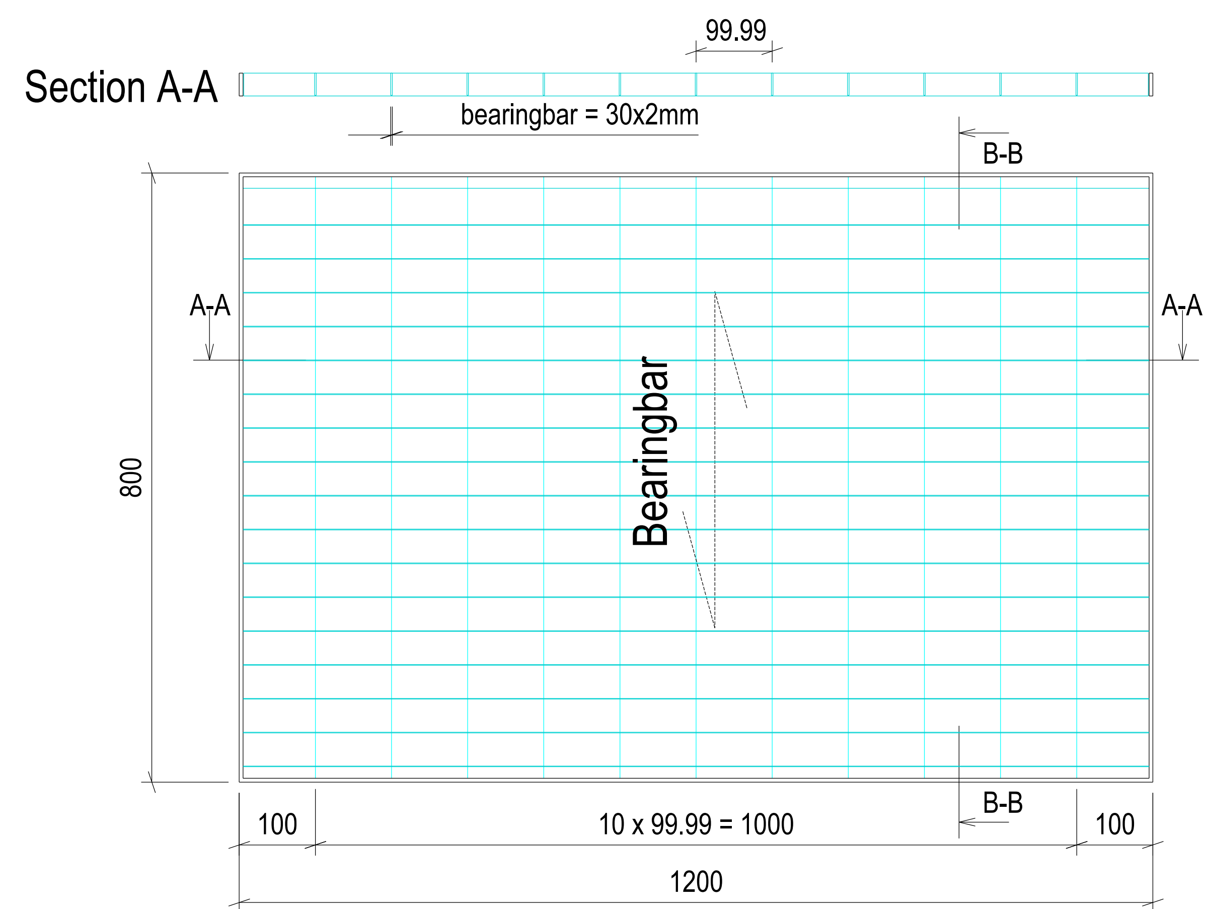
TYPE RL 30-2/ 99.99x44.44 Louvre 55-2/ 60°
